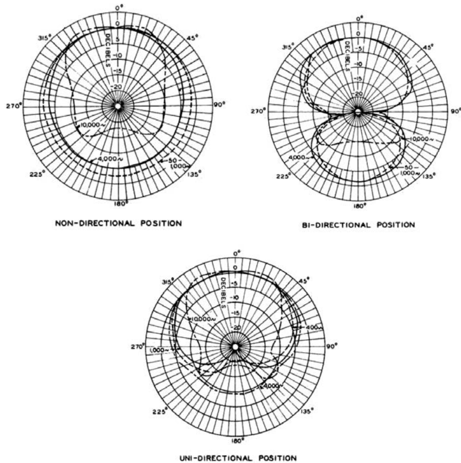
Figure 29 - Polar responses of the RCA 77 D microphone in its three configurations
