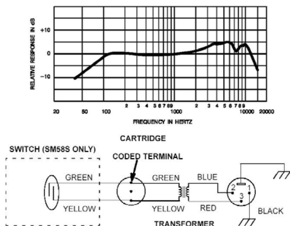
Figure 31 – Frequency response and circuit of the SM58 ® microphone (Copyright Shure Incorporated. Used with permission.)
