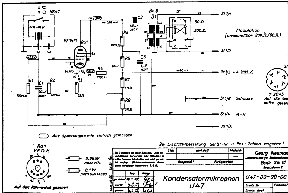
Figure 35 - Circuit of the U47
