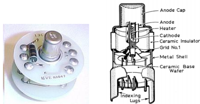
Figure 37 - 13CW4 Nuvistor and the assembly which replaced the VF14(M) valve
